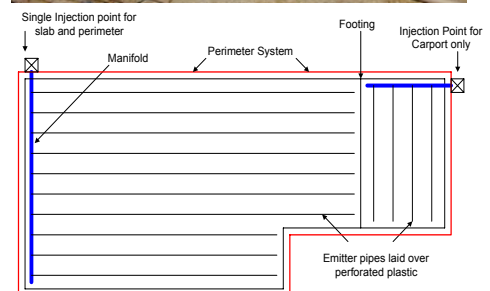
Plans of ALTIS Premium System under concrete-on-ground of new House and Carport - Plan View
